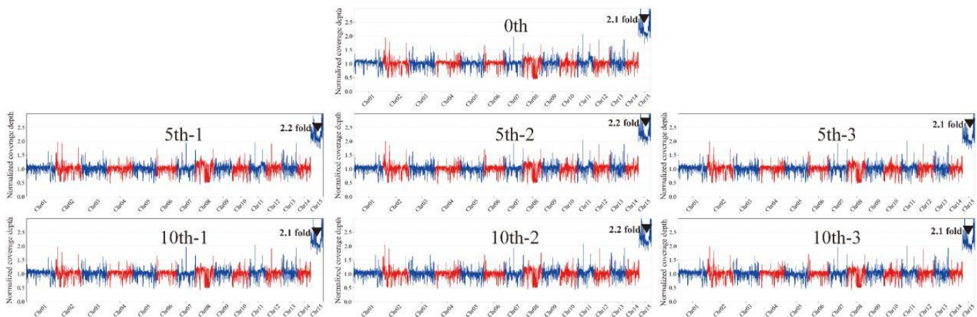
Figure S25. Genome coverage of strain 776 during subculturing. Sequencing of the starting strain and the 5th and 10th generations is shown. Numbers indicate AC dosage inferred from normalized coverage.
