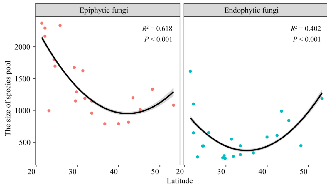
Figure S7 Latitudinal pattern of phyllosphere epiphytic and endophytic fungal species pools.
