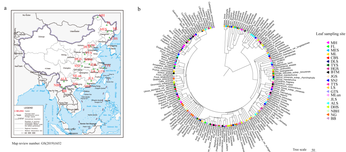
Figure S1 Distribution of leaf samples collected from 172 plant species in 21 Chinese forest sites. a Distribution of 21 sampling forest sites. b Phylogenetic tree of 172 host plant species used in this study. Information of sampling sites is listed in Table S1. BB, Bubeng; NG, Nonggang; NBH, Nabanhe; DHS, Dinghushan; ALS, Ailaoshan; JLS, Jiulianshan; MLun, Mulun; GTS, Gutianshan; LS, Lushan; TTS, Tiantongshan; SNJ, Shennongjia; JGS, Jigongshan; BTM, Baotianman; HGS, Huangguanshan; TYS, Taiyueshan; DLS, Donglingshan; CBS, Changbaishan; ML, Muling; MES, Maoershan; FL, Fenglin; MH, Mohe.
