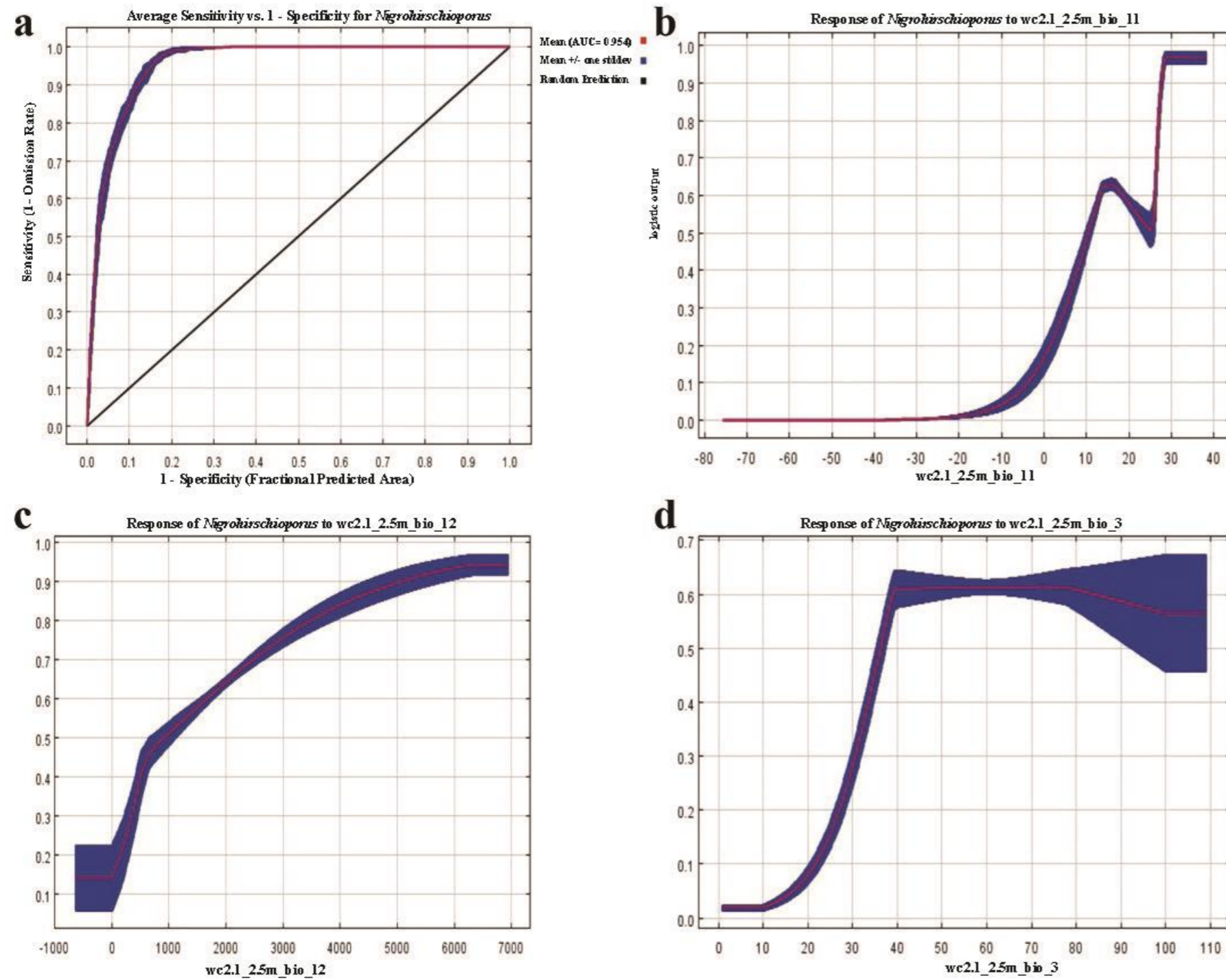
Figure S4. Maxent model of Nigrohirschioporus a) The receiver operating curve, b) The response curves for the Mean Temperature of Coldest Quarter (Bio11), c) The response curves for the Annual Precipitation (Bio12), d) The response curves for the Isothermality (Bio3)
