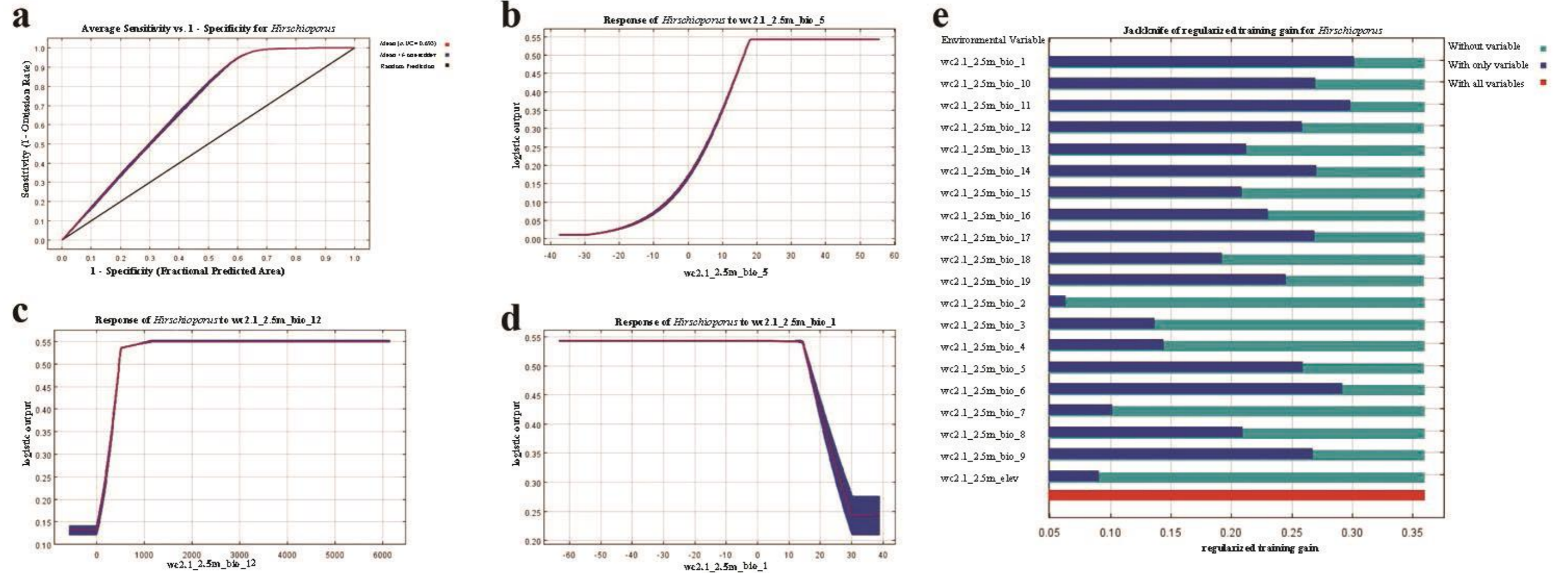
Figure S1. Maxent model of Hirschioporus a) The receiver operating curve, b) The response curves for the Max Temperature of Warmest Month (Bio5), c) The response curves for the Annual Precipitation (Bio12), d) The response curves for the Annual Mean Temperature (Bio1), e) Jackknife analysis of Hirschioporus
