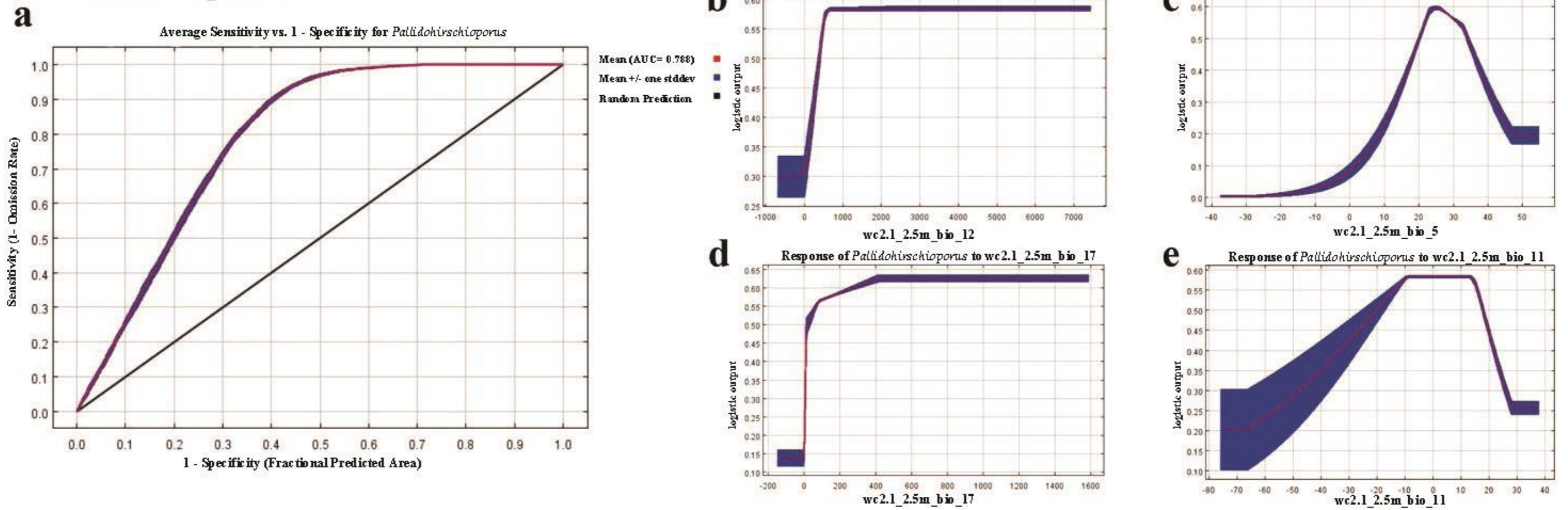
Figure S2. Maxent model of Pallidohirschioporus a) The receiver operating curve, b) The response curves for the Annual Precipitation (Bio12), c) The response curves for the Maximum Temperature of Warmest Month (Bio5), d) The response curves for the Precipitation of Driest Quarter (Bio17), e) The response curves for the Mean Temperature of Coldest Quarter (Bio11)
