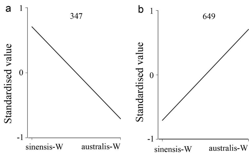
Figure S7. K-means cluster analysis of metabolites from S. sinensis (a) and S. australis (b)
