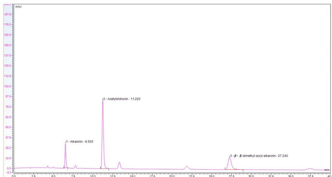
Supplementary Figure S1: Chromatogram of standard reference substances.
