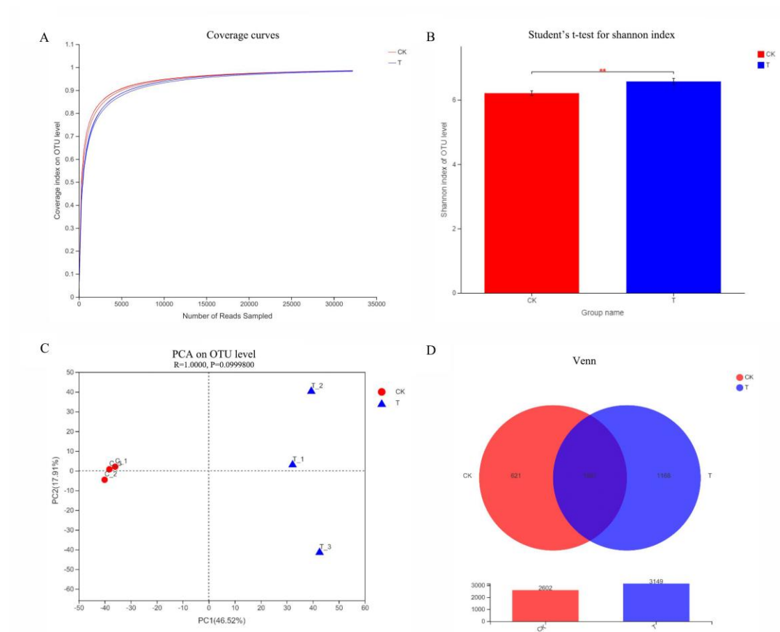
Figure S1: Diversity analysis of bacteria at the operational taxonomic unit (OTU) level in all samples. (A) Alpha diversity analysis of the coverage curves. (B) Alpha diversity analysis of the Shannon index. (C) PCA analysis between different groups. (D) Venn diagram of bacterial community composition between different groups.
