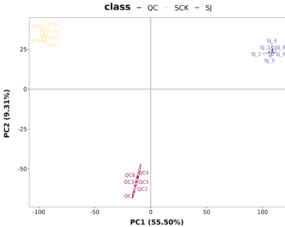
Fig. S4. The principal component analysis of the data from SCK and SJ.
