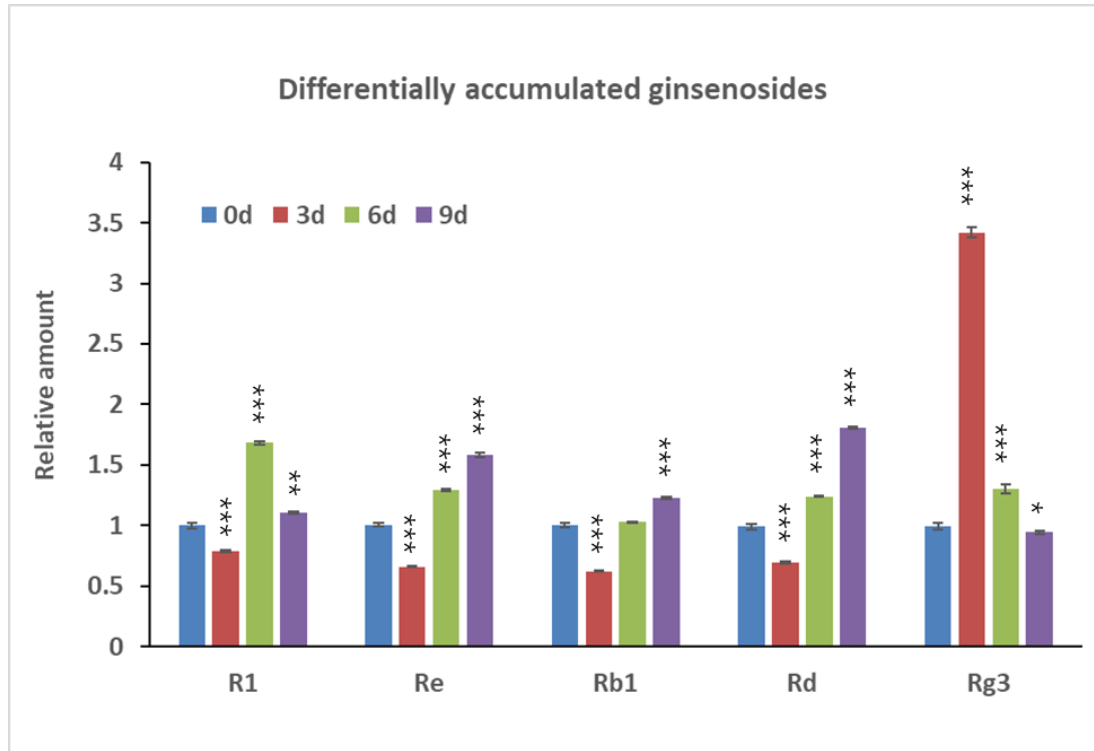
Fig. S2. Differentially accumulated ginseng saponins in P. notoginseng after interaction with A. cristatus at different time (*, p < 0.05 ; **, p < 0.01 ; ***, p < 0.001 ).
