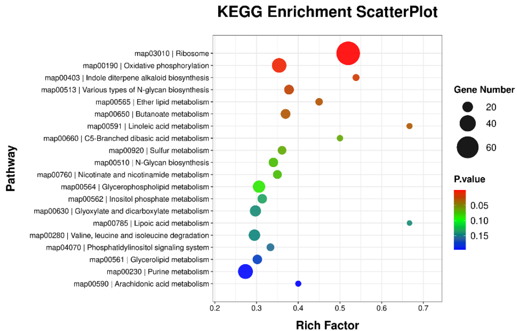
Fig. S9. GO and KEGG analysis of DEGs. (a) GO analysis of differentially expressed genes in A. cristatus after one week interaction with P. notoginseng roots. (b) KEGG analysis of differentially expressed genes in A. cristatus after one week interaction with P. notoginseng roots.
