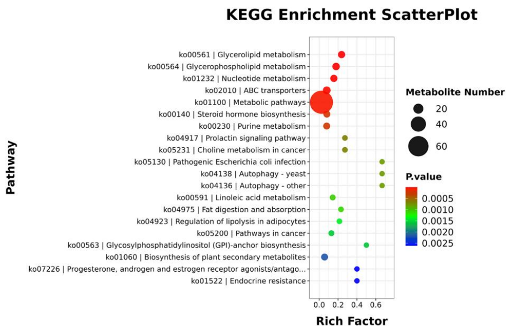
Fig. S5. Differentially changed features in A. cristatus treated P. notoginseng (SJ) and the untreated control (SCK). (a) Numbers of differentially changed features in SJ an SCK. (b) KEGG analysis of differentially accumulated metabolites in P. notoginseng during interaction with A. cristatus .
