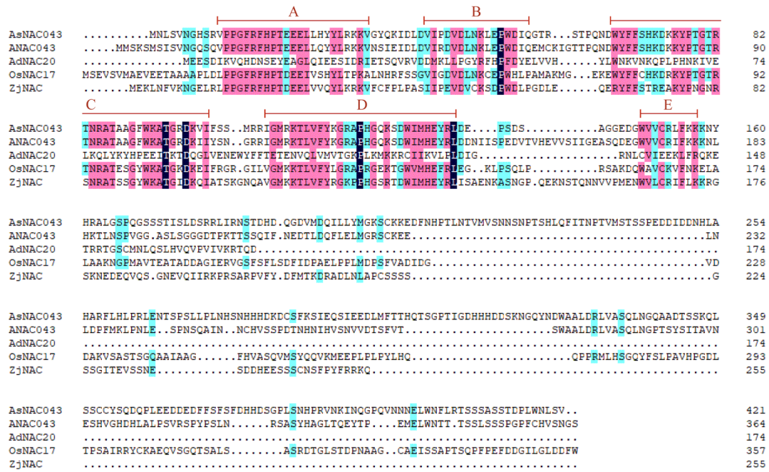
Fig.S5. Multiple alignment of amino acid sequences from AsNAC043. A-E represent the five subdomains of NAC. ANAC043 (NP_182200.2), AdNAC20 (TRINITY_DN81887_c0_g1), OsNAC17 (BAS84001.1), ZjNAC (XP_015902286.2), with accession numbers in parentheses.
