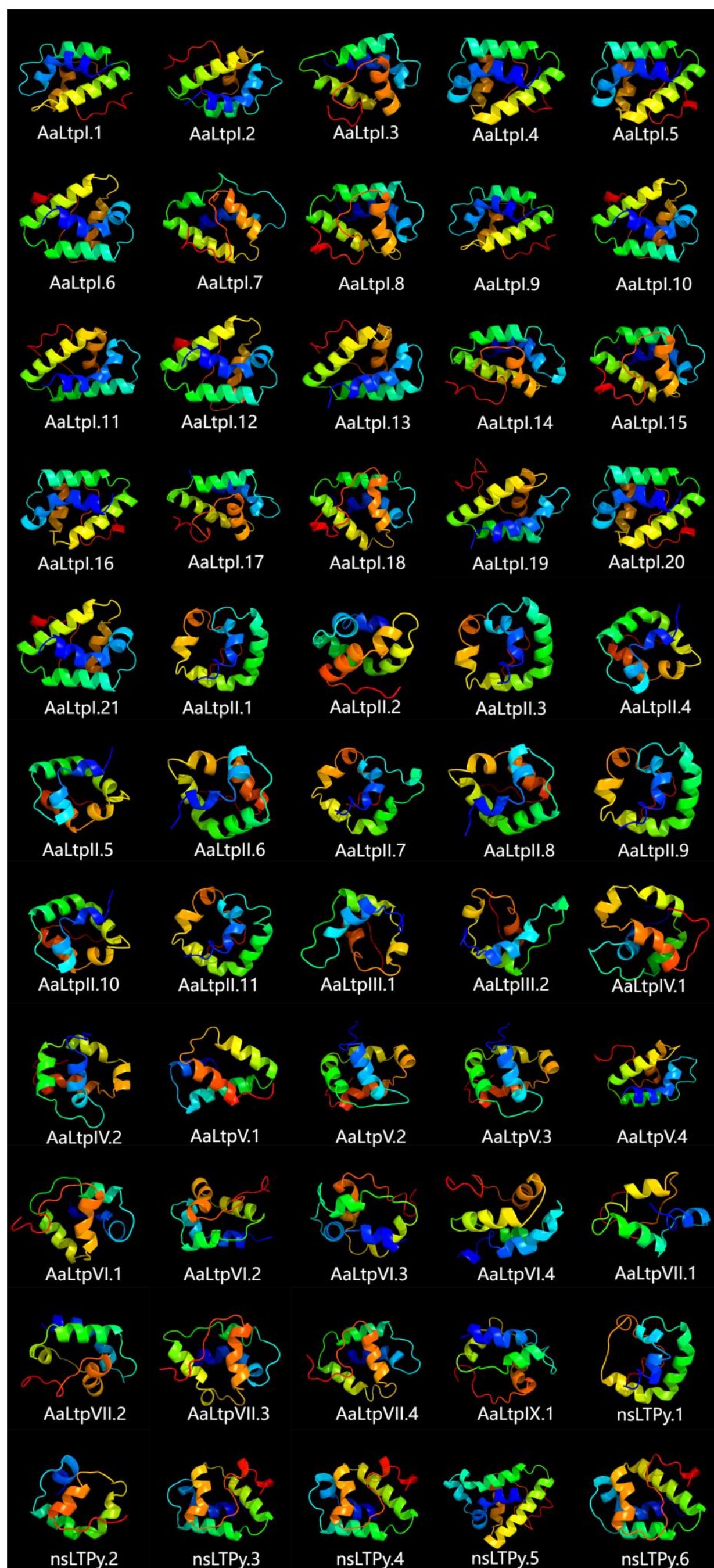
Figure S1 Three-dimensional structures of the mature AaLTPs predicted by Phyre2
