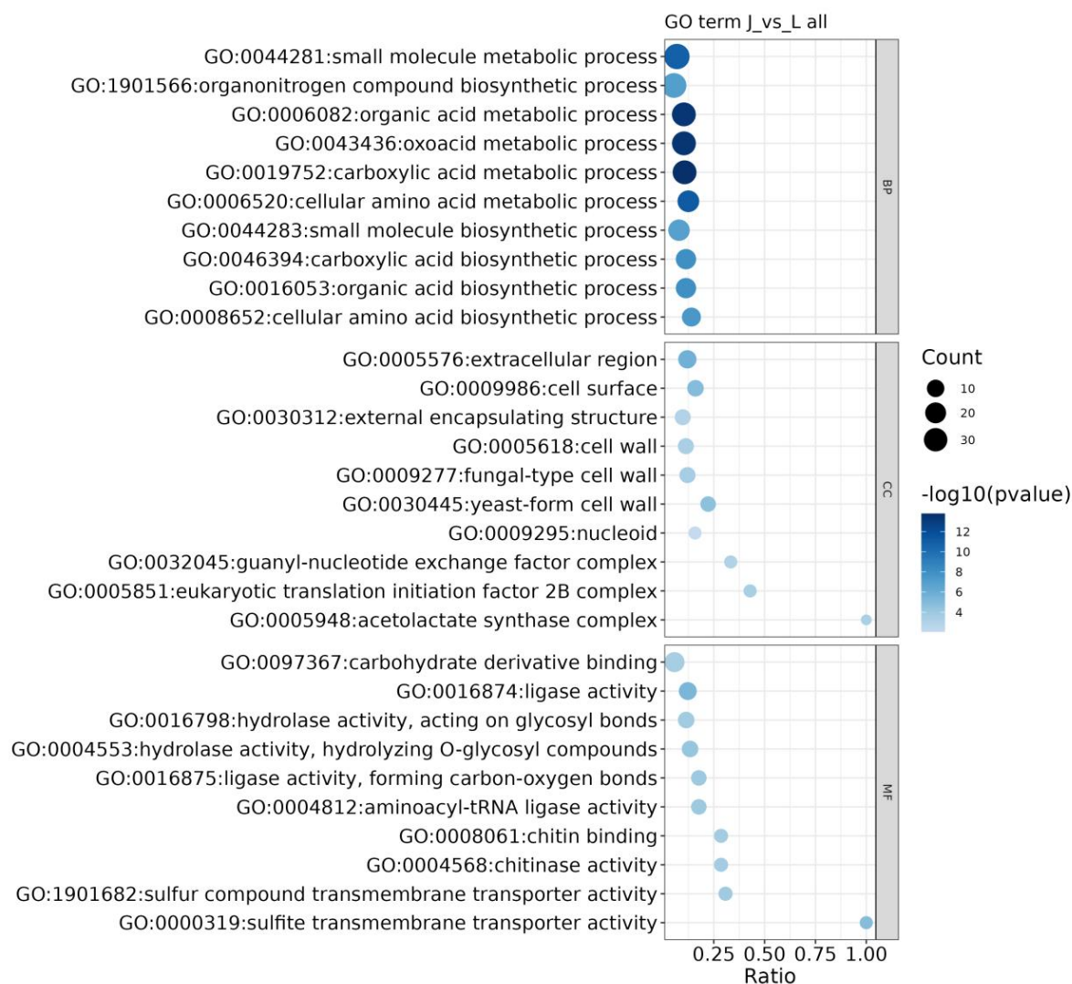
Fig. S13 GO enrichment analysis of the DEGs from 5-AC treatment group
