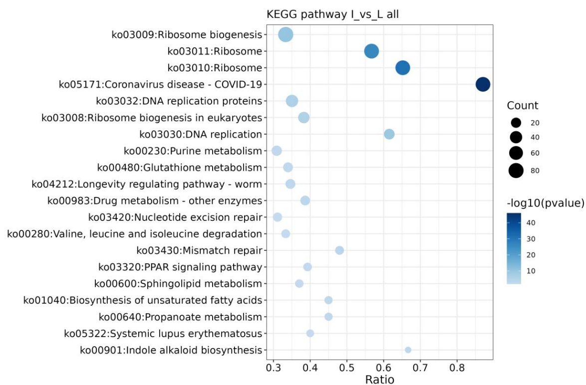
Fig. S12 KEGG enrichment analysis of DEGs from MeJA treatment group
