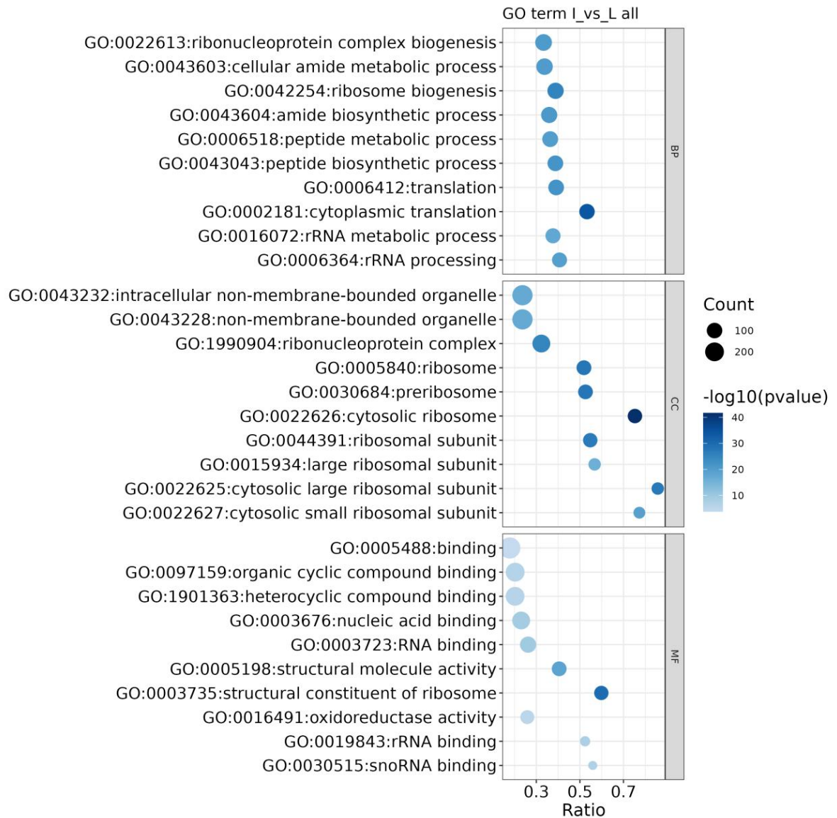
Fig. S11 GO enrichment analysis of the DEGs from MeJA treatment group
