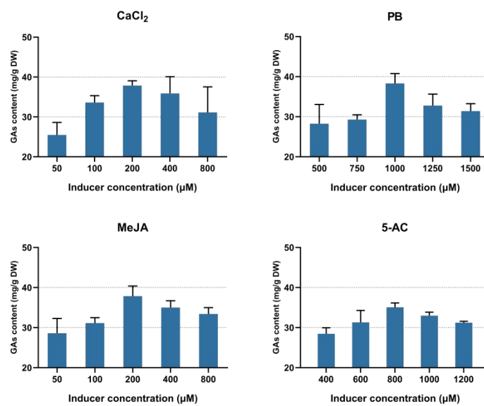
Fig. S1 Effect of CaCl 2 , PB, MeJA and 5-AC at various concentrations on GAs content based on RSM
