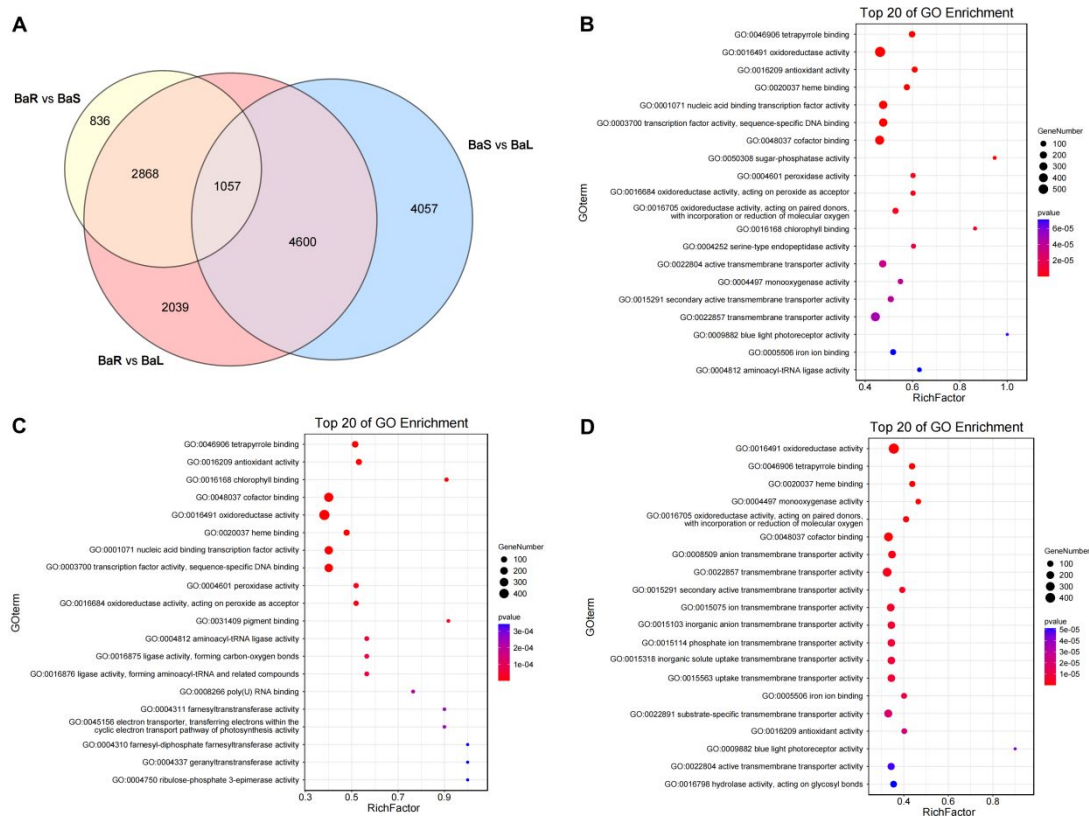
Supplementary Figure S3. GO enrichment analysis of DEGs in different comparisons. (A) Venn diagram of up-regulated DEGs in different comparisons. (B-D) Scatterplot of GO enrichment of DEGs that were enriched in the molecular function aspect (top 20) (BaR vs BaL, BaS vs BaL, and BaR vs BaS, respectively).
