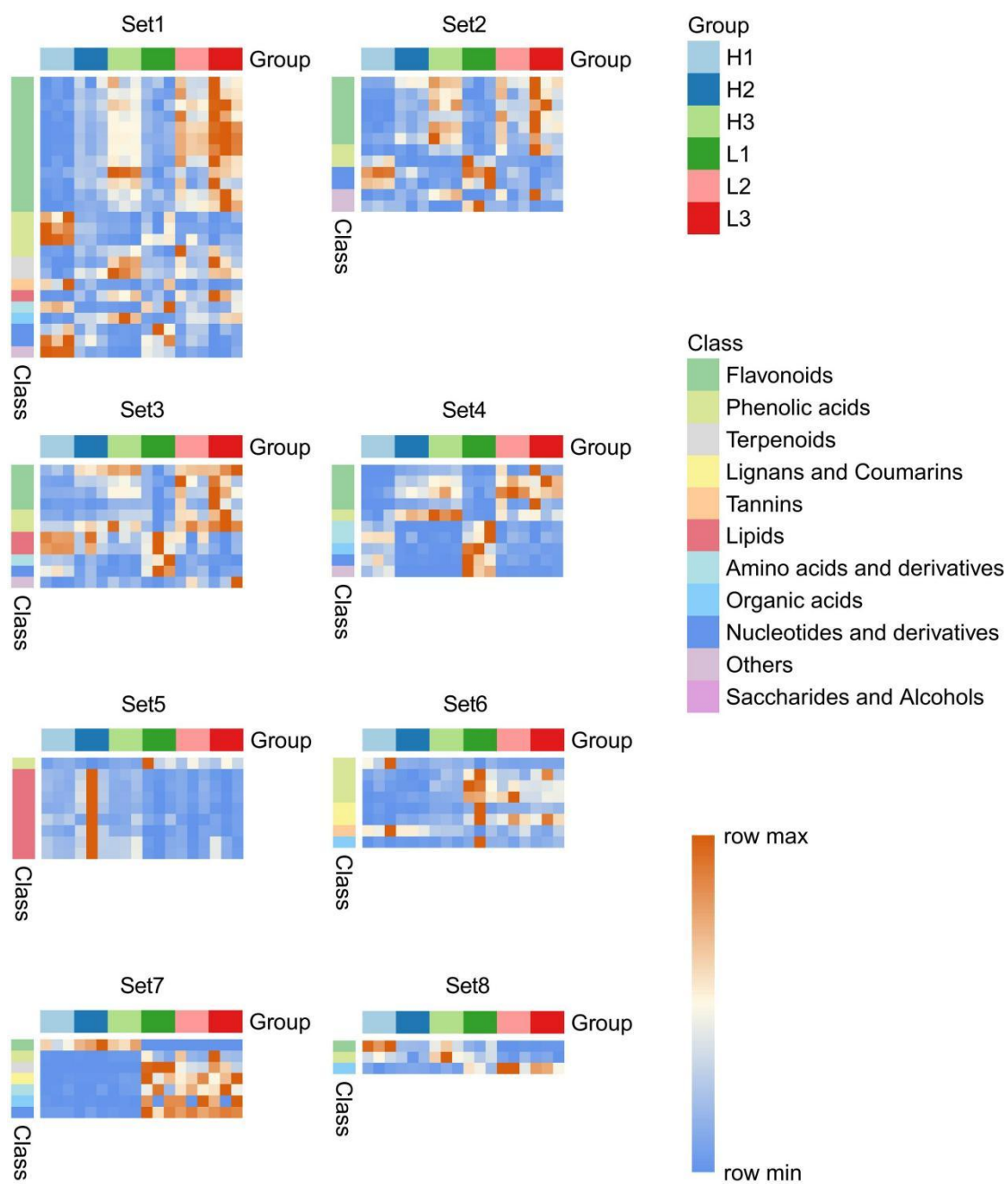
Supplementary Fig. S4 Expression profiles of different DEM sets.
