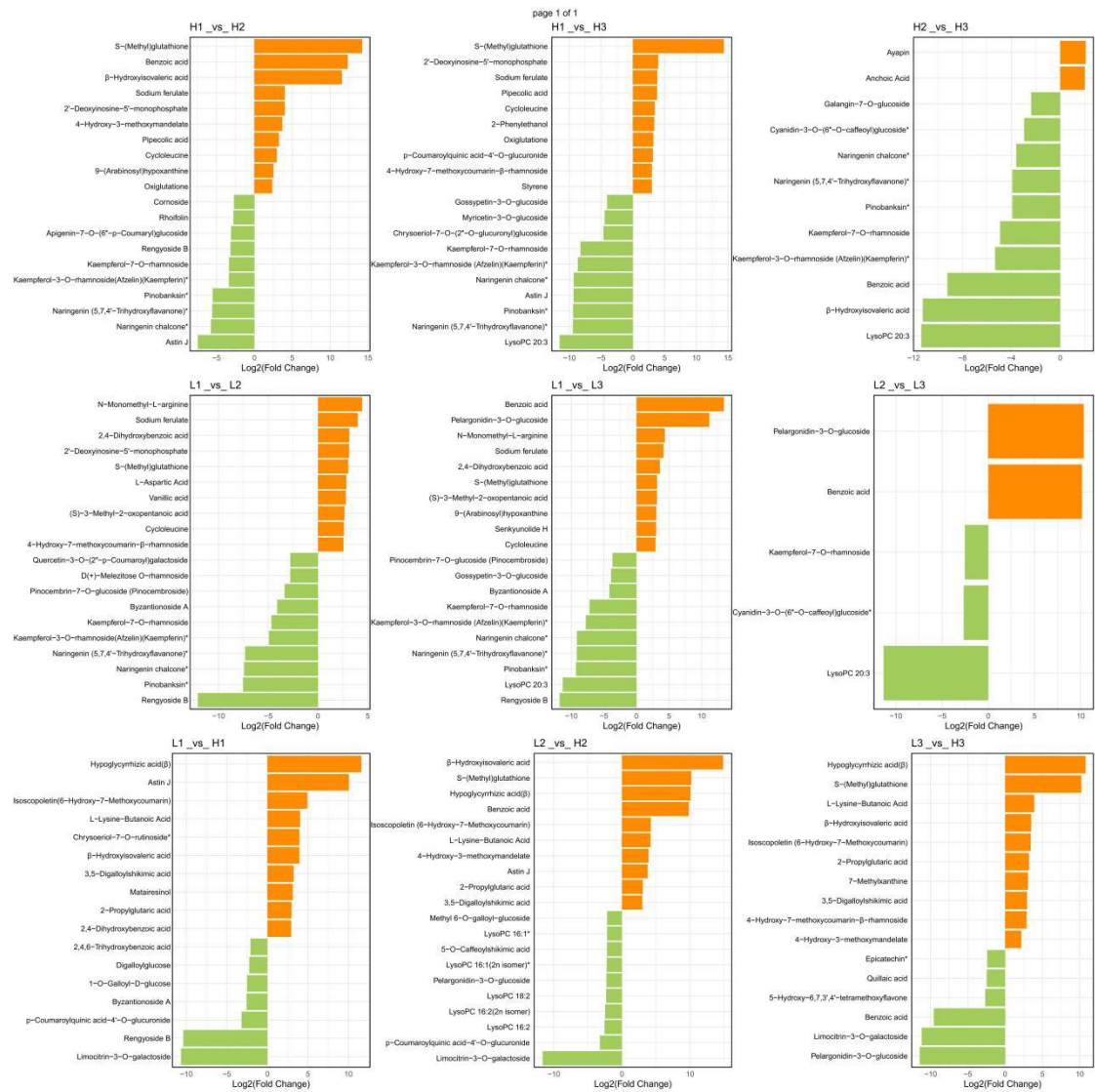
Supplementary Fig. S3 Log2(Fold Change) for DEMs with the most significant differences across comparison groups.
