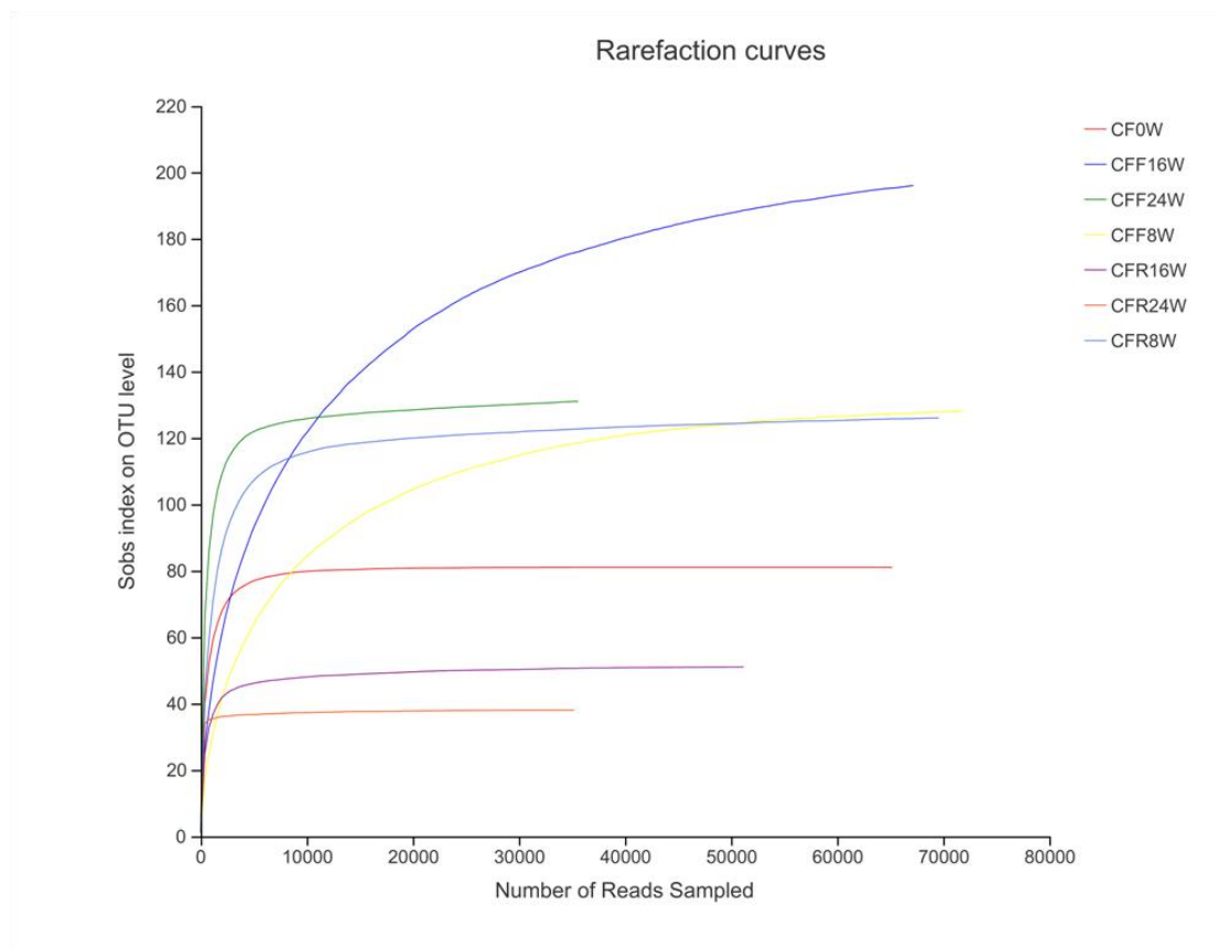
Figure S1 Rarefaction curves for OTU in seven CF samples
