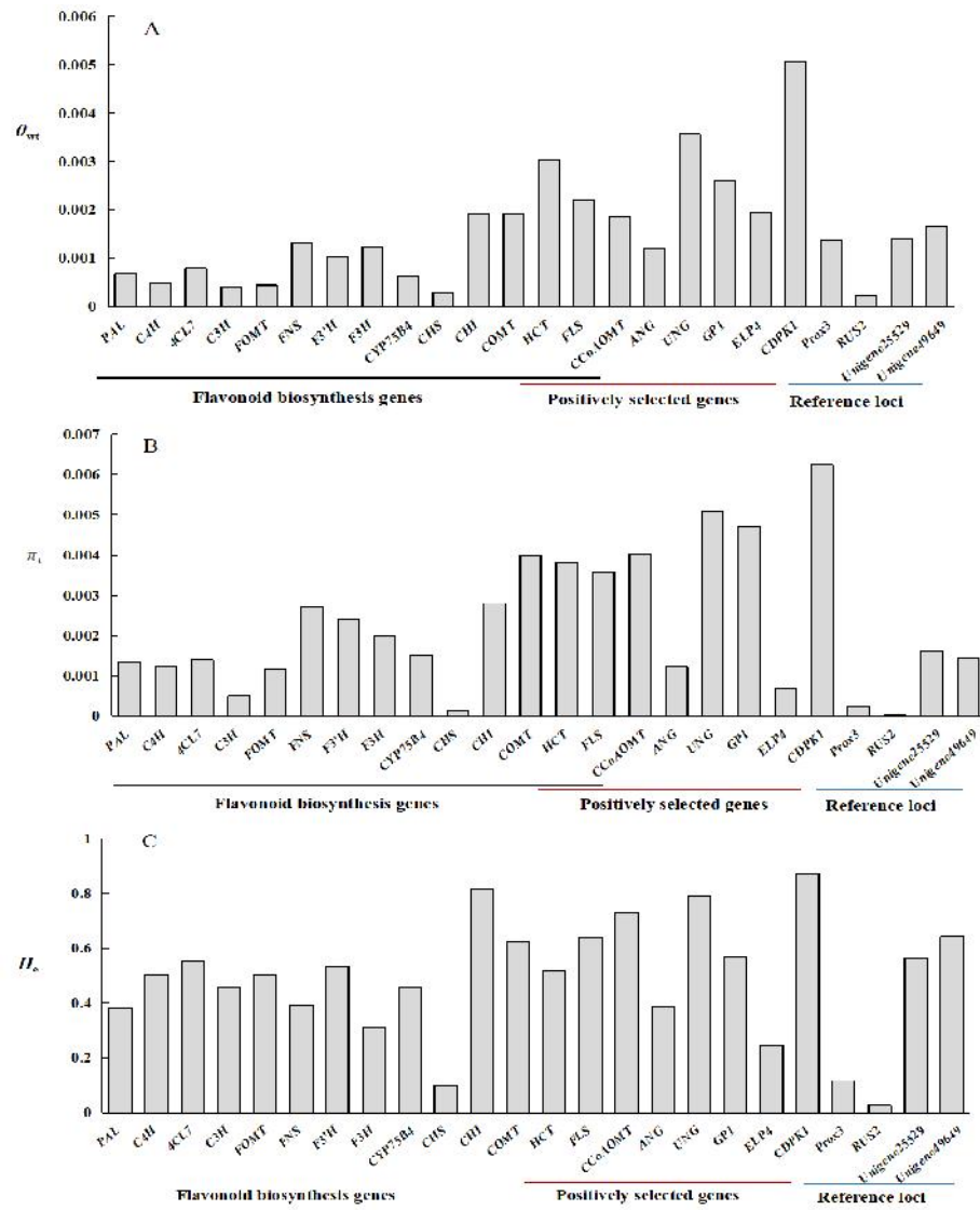
Figure S3 The nucleotide diversity of flavonoid biosynthesis genes, positively selected genes and the reference loci in different altitude groups of A. squarrosun . A: Watterson's parameter; B: Nucleotide diversity; C: Haplotypic diversity.
