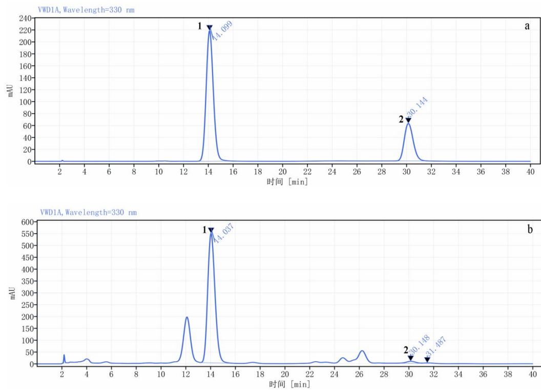
Figure S4 HPLC-UV map of reference substance (a) and test substance for C. deserticola parasitizing S. tragus (b). 1. echinacoside, 2. acteoside.
