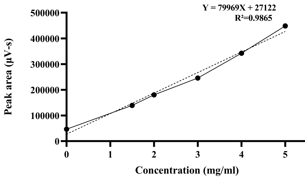
Figure S1. The standard curve between the HPLC peak area and betanin content (0, 1.5, 2, 3, 4, and 5 mg/ml). A linear regression was observed between the peak area and betanin contents at 0-5mg ( R^2 = 0.9865 ).
