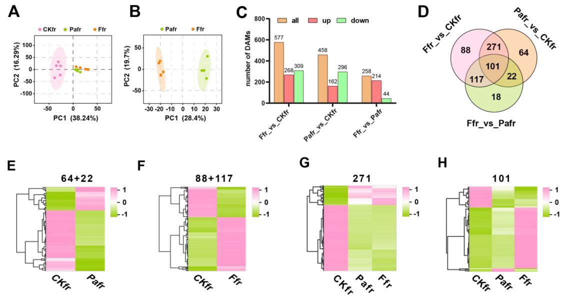
Fig. S5: The common and differential effects of inoculation with F9 and Pa on the distribution of metabolites in A. lancea fibrous roots. The first principal component (PC1) in PCA analysis explained 38.24% of the difference between F9, Pa, and CK (A). PC1 explained 28.4% of the difference between F9 inoculation and Pa inoculation group (B). Further, differential accumulation metabolites (DAMs) number (C) and Venn analysis (D) from pairwise comparisons among F9, Pa inoculation groups and the control were showed. Based on Venn analysis, the specific (E-F, H) or common (G) DAMs accumulated in A. lancea fibrous roots caused by F9 or Pa were visualized by heat map. Abbreviation, "fr" fibrous root.
