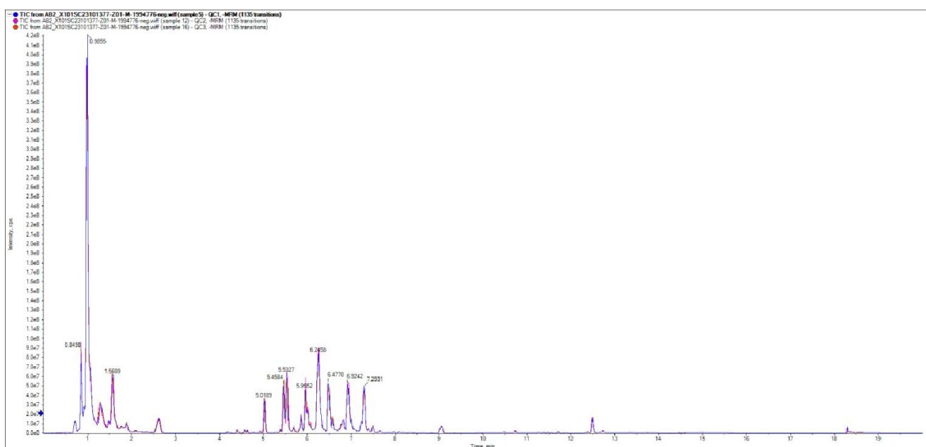
Supplementary Figure S5. Total ion chromatograms (TICs) of QC samples in both positive (a) and negative (b) ion modes.
