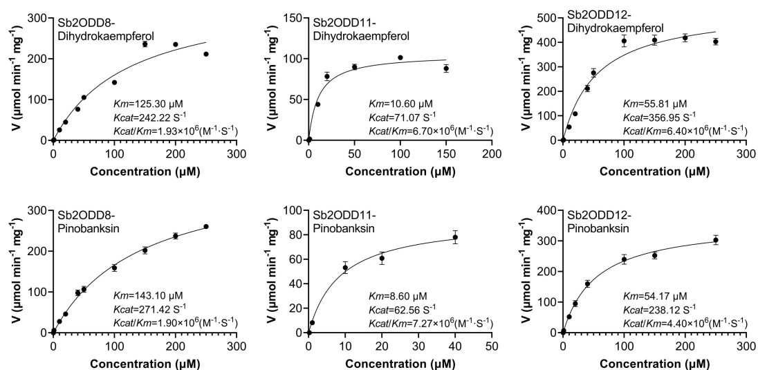
Fig. S2 Enzymatic kinetic curve of Sb2ODDs.
