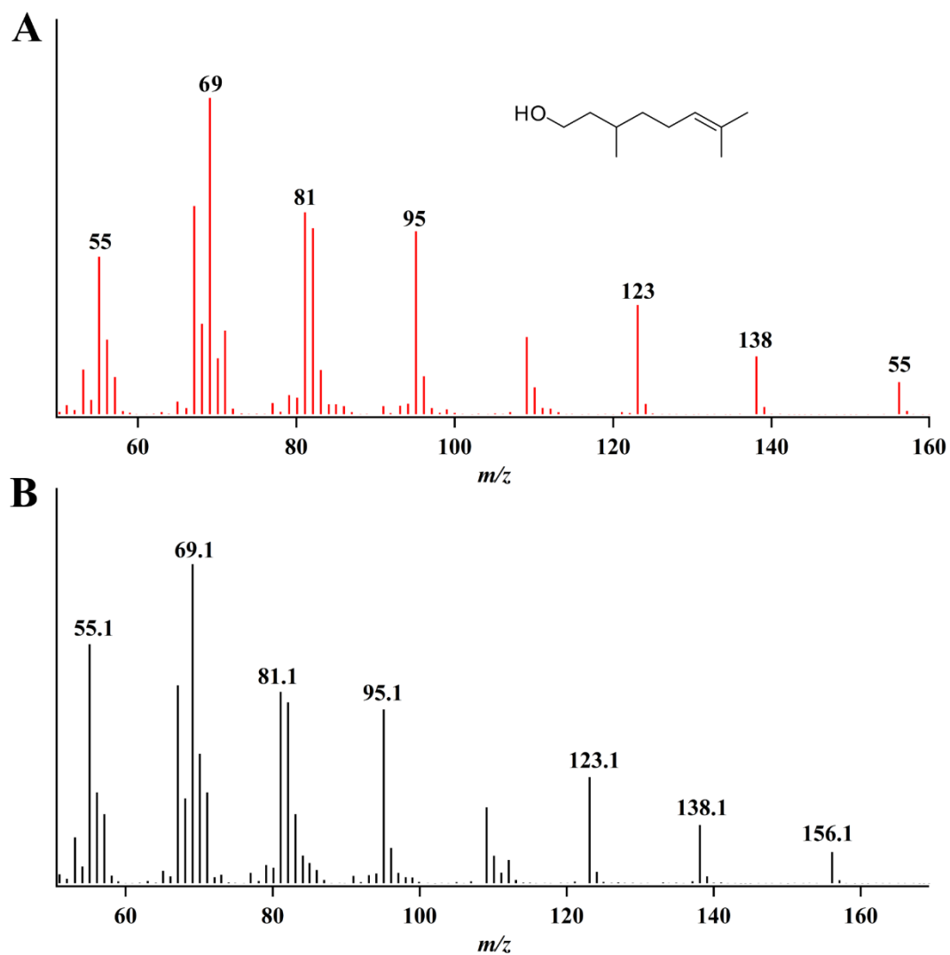
Figure S5. The mass spectrum of citronellol. A. The mass spectrum of standard citronellol. B. The mass spectrum of the major product of PfTPS47-PA.
