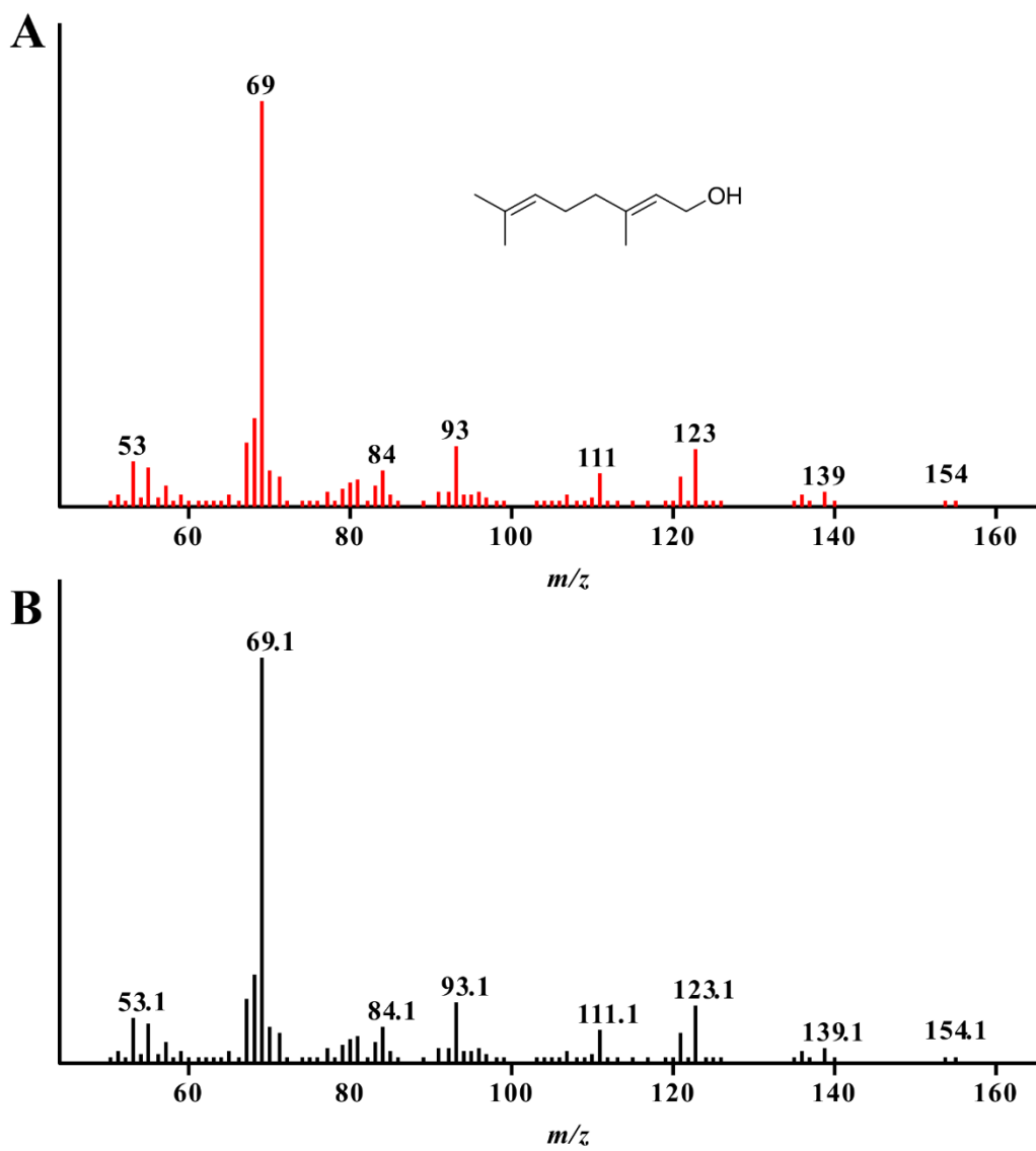
Figure S6. The mass spectrum of geraniol. A. The mass spectrum of standard geraniol. B. The mass spectrum of the minor product of PFTPS47-PA.
