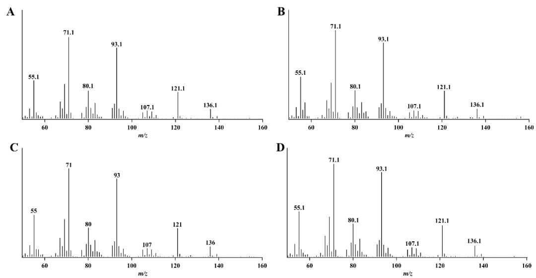
Figure S2. The mass spectrum of the product of PfTPS46-PK, PfTPS18-PA and PfTPS49-PA.
