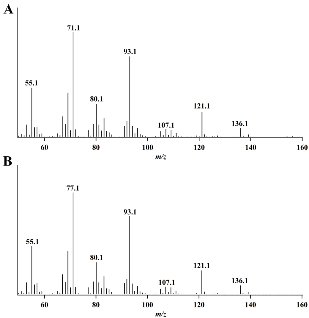
Figure S4. The mass spectrum of the product of the crude proteins of PfTPS18-PA.
