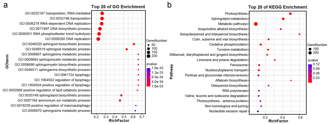
Figure S4 GO and KEGG enrichment terms of rapid evolution gene families in P. ternata
