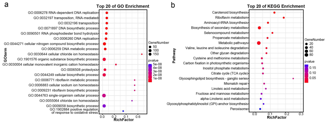
Figure S5 GO and KEGG enrichment terms of specific gene families in P. ternata (Biological process)
