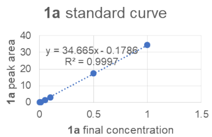
Figure S26. Calibration curves for 1a and 2a .
