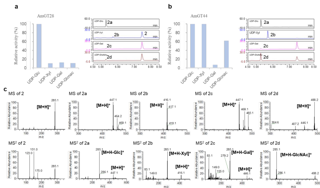
Figure S21. UHPLC/UV and UHPLC/MS analysis of AmGT28/AmGT44 catalytic reaction mixtures for compound 2 with UDP-Glc, UDP-Xyl, UDP-Gal and UDP-GlcNAc. (a, b) UHPLC chromatogram of the reaction mixtures. (c) MS and MS/MS spectra for 2 , 2a , 2b , 2c and 2d .
