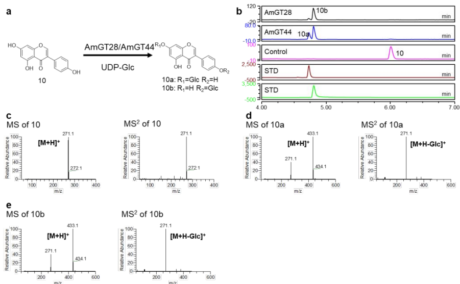
Figure S10. UHPLC/UV and UHPLC/MS analysis of AmGT28/AmGT44 catalytic reaction mixtures for compound 10 with UDP-Glc. (a) Reaction scheme. (b) UHPLC chromatogram of the reaction mixtures. Control, reactions conducted using boiled protein; STD, reference standard. (c) MS and MS/MS spectra for 10 . (d) MS and MS/MS spectra for 10a . (e) MS and MS/MS spectra for 10b .
