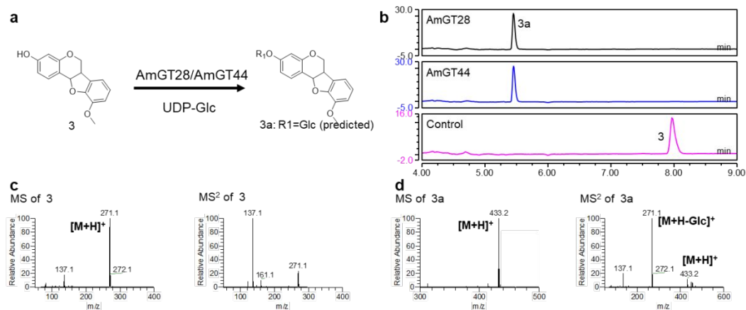
Figure S3. UHPLC/UV and UHPLC/MS analysis of AmGT28/AmGT44 catalytic reaction mixtures for compound 3 with UDP-Glc. (a) Reaction scheme. (b) UHPLC chromatogram of the reaction mixtures. Control, reactions conducted using boiled protein; STD, reference standard. (c) MS and MS/MS spectra for 3 . (d) MS and MS/MS spectra for 3a .
