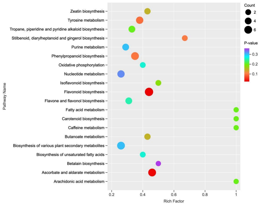
Figure S13. KEGG enrichment analysis of differential metabolites between P. cernua and P. chinensis .
