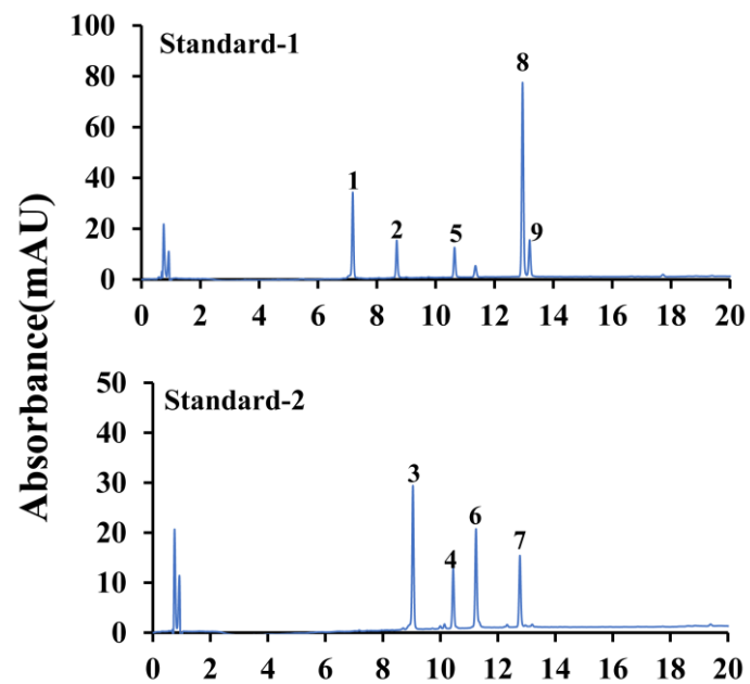
Figure S4. Chromatograms of nine flavones standard analyzed by LC-MS. Compounds identified in chromatographic peaks: 1, Scutellarin; 2, Scutellarein; 3, Baicalin; 4, Wogonoside; 5, Apigenin; 6, Baicalein; 7, Wogonin; 8, Chrysin; 9, Oxoylin A.
