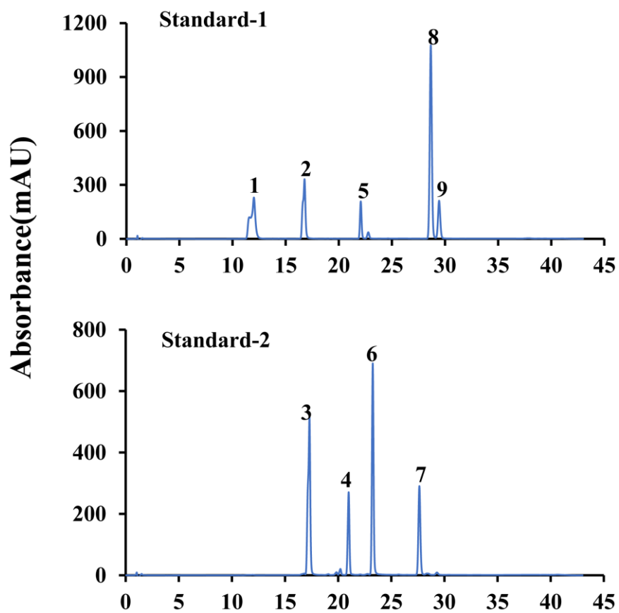
Figure S1. HPLC chromatograms of nine flavones standard. Compounds identified in chromatographic peaks: 1, Scutellarin; 2, Scutellarein; 3, Baicalin; 4, Wogonoside; 5, Apigenin; 6, Baicalein; 7, Wogonin; 8, Chrysin; 9, Oxoylin A.
