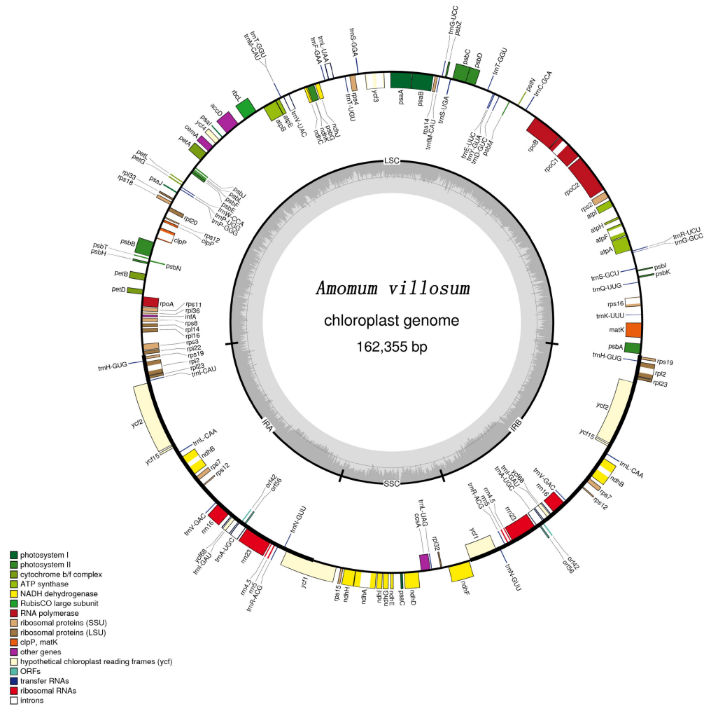
Figure S1. Gene map of the complete chloroplast genome of A. villosum . Genes located on the inside and outside of the circle are transcribed clockwise and counterclockwise, respectively. The inner circle indicates the GC and AT content.
