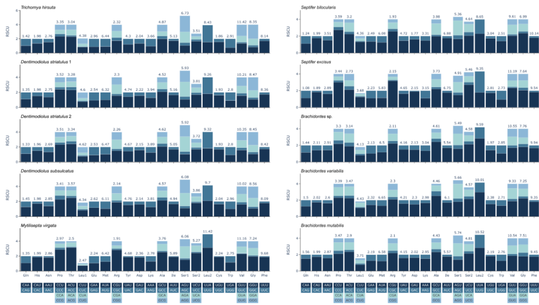
Figure S5. Relative synonymous codon usage (RSCU) of the ten mitogenomes
