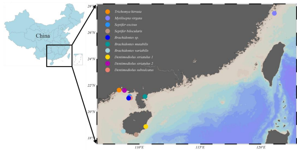
Figure S1. Distribution map of the nine Mytilidae species from coastal China. The dots represent sampling sites, with different species marked with different colors.
