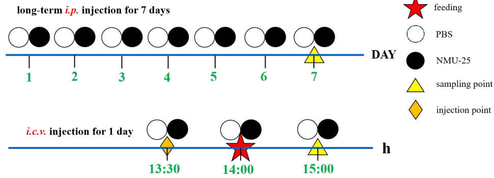
Fig. S2 Long-term i.p. and i.c.v. injection experiments
