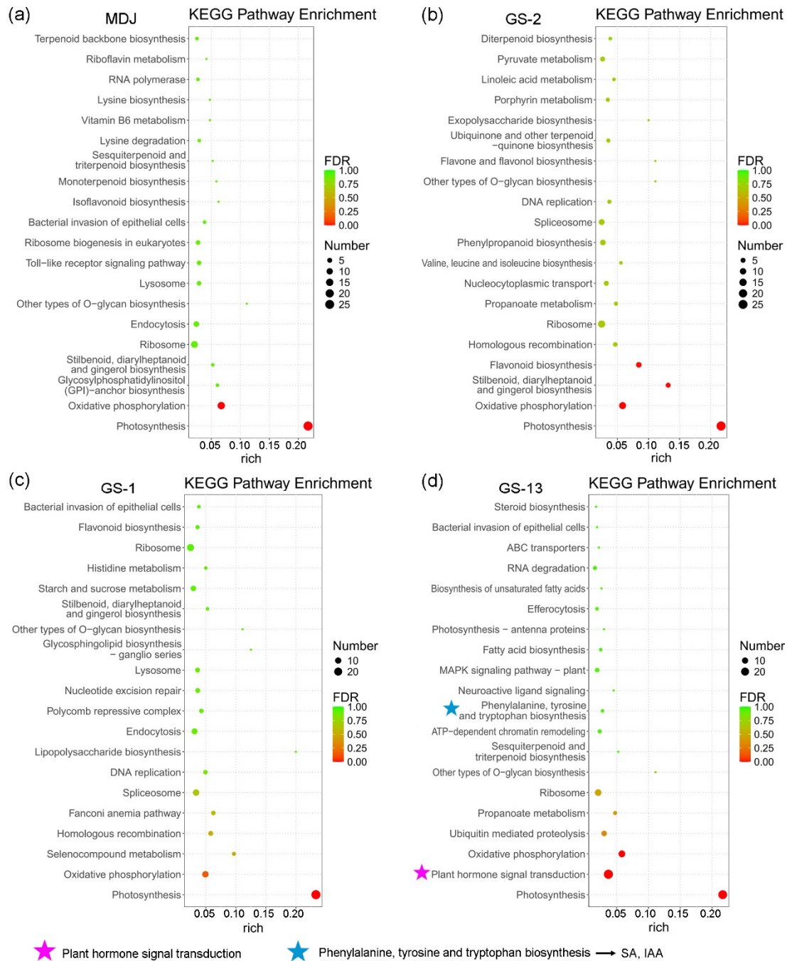
Fig. S5 KEGG pathway enrichment analysis of genes covered by copy number variations (CNVs) in soybean accessions MDJ (a), GS-2 (b), GS-1 (c), and GS-13 (d). Stars mark phytohormone-related pathways: yellow star for brassinosteroid biosynthesis (BR), black star for zeatin biosynthesis (CK), purple star for plant hormone signal transduction, blue star for phenylalanine, tyrosine and tryptophan biosynthesis (SA, IAA), green star for phenylalanine metabolism (SA).
