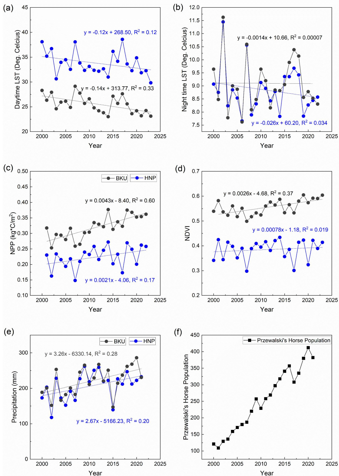
Fig. S1. Interannual variation characteristics of the growing season in HNP and BKU; (a) Daytime LST from 2000 to 2023, (b) Night time LST from 2000 to 2023, (c) Net Primary Production (NPP) from 2001 to 2022, (d) Normalized Differences Vegetation Index (NDVI) from 2000 to 2023, (e) Precipitation from 2001 to 2021, and (f) the Przewalski's horse population in HNP from 2000 to 2021.
