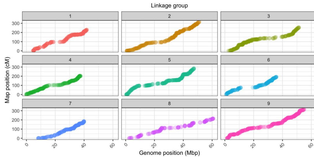
Supplementary Figure S3. Scatter plot of the map position (cM) versus the genome position (Mbp) of the markers showing synteny between them in nine linkage groups generated from the St. Augustinegrass Raleigh selfing population. cM = centimorgan, Mbp = mega base pair.
