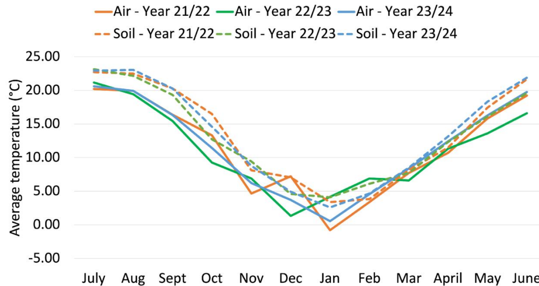
Supplementary Figure S1. Trends for the average monthly air (2 m above ground) and soil (10 cm underground) temperatures for the 21/22, 22/23, and 23/24 seasons at the Upper Mountain Research Station (Laurel Spring, NC).
